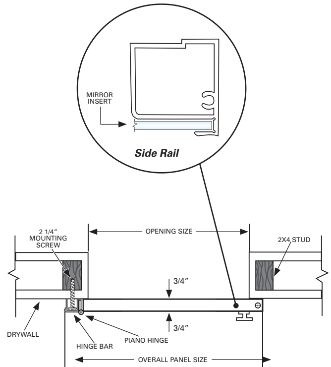
Technical Illustration
