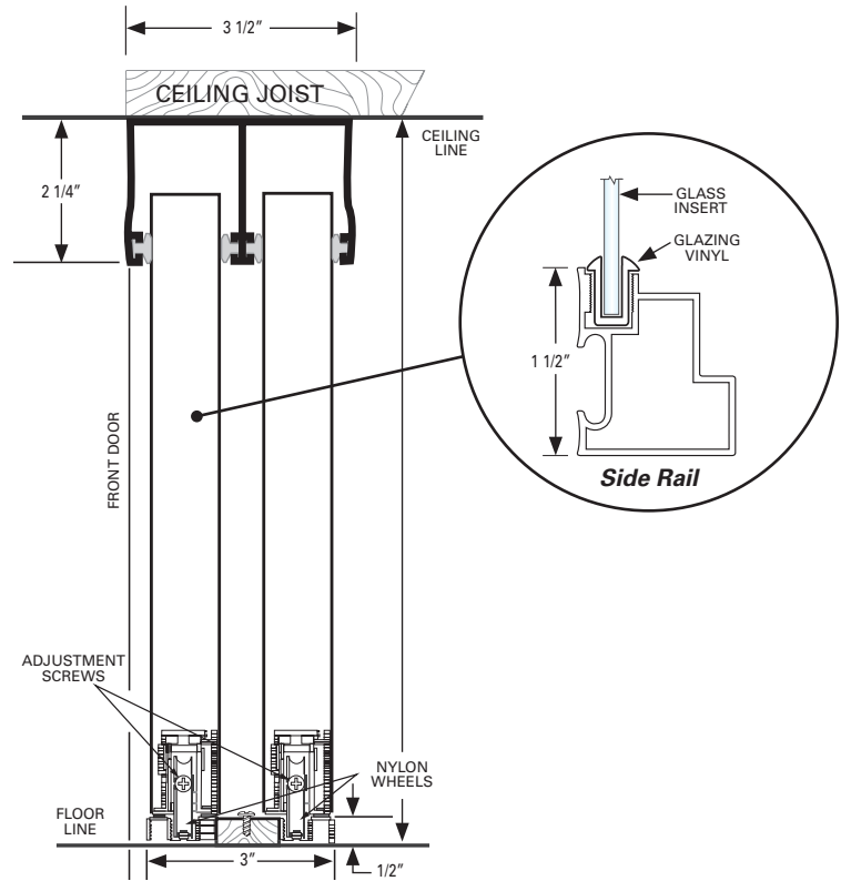
Technical Illustration
